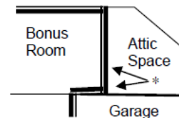
Building Segment More Than 60° to Horizontal - Wall.
