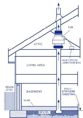
Active System In Basement or with Slab-On-Grade
