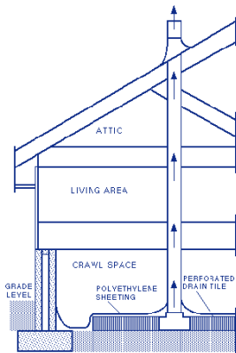
Passive System In Crawlspace
