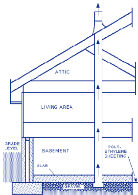
Passive System In Basement with Slab-On-Grade
