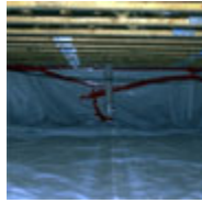
Example of a crawlspace without mold or water problems. The site is well drained. The crawlspace has a vapor barrier over the earth, is air-sealed, and insulated on the walls. (photo courtesy of Terry Brennan)
